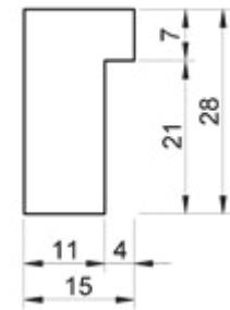
profile dimensions
